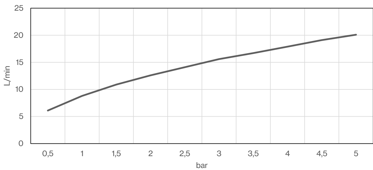
QS3200 built-in part only (flowrate L/min)
