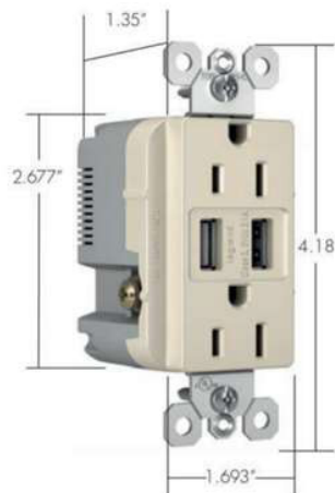
Dimensions of typical duplex inserts
