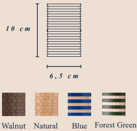
Cylinder
