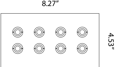
VERTICAL 8 BUTTON FITS 4 GANG BOX
