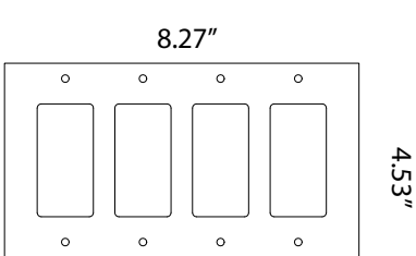
4 GANG
