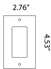
1 GANG
