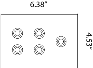
VERTICAL 5 BUTTON FITS 3 GANG BOX
