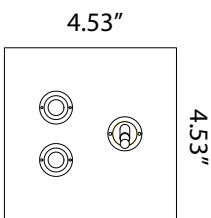
VERTICAL 2 BUTTON 1 TOGGLE FITS 2 GANG BOX
