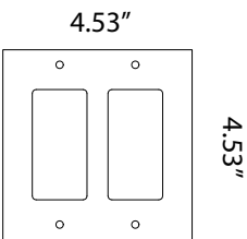
2 GANG
