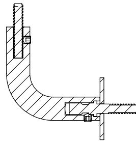
SECTION E-E SCALE 1 : 2
